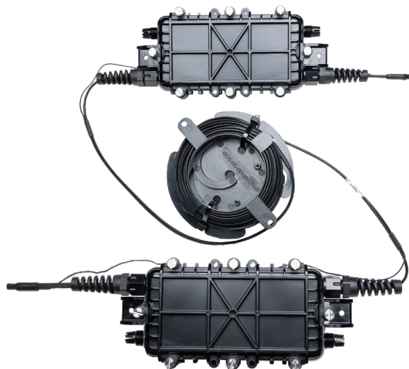
LOC-DROP® Fast Repair Kit
